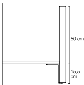
Front mounted fitting article no. 5132
