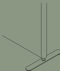
Rounded adjustable foot article no. 5121
