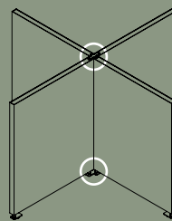
Connecting bracket article no. 5223
