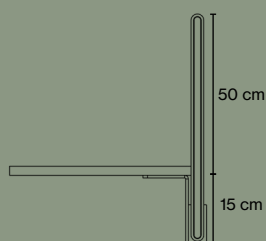
Front mounted fitting article no. 3032
