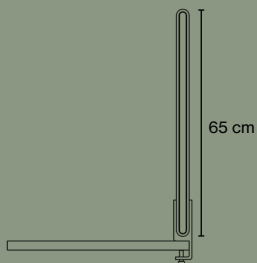
Clamp fitting article no. 3030
